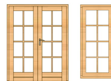
PE50H 1510 x 1935 PE50XL 1510 x 2070
