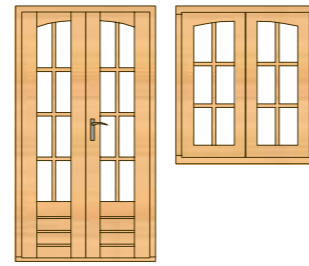
PR30 1000 x 1800 PR30H 1000 x 1935
