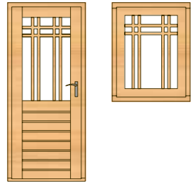
PJ04 770 x 1800 PJ04H 770 x 1935
