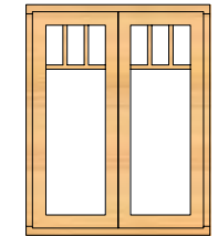
PE41 1210 x 1800 PE40 1210 x 1530 PE41H 1210 x 1935
