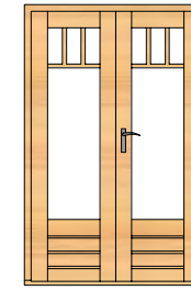
PE41 1210 x 1800 PE40 1210 x 1530 PE41H 1210 x 1935
